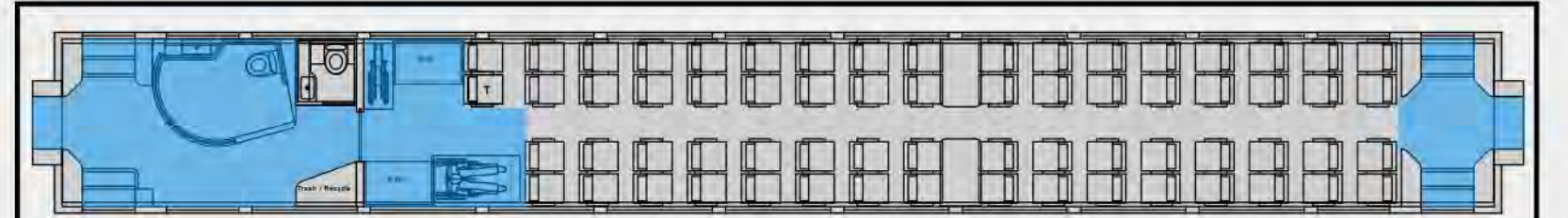
HIGH CAPACITY COACH (37" pitch) - 66 C / 1 MOB *2x DOORS
