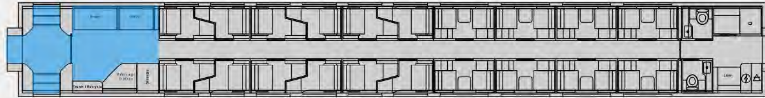
STANDARD SLEEPER - 12 S / 7 R / 1 Crew
