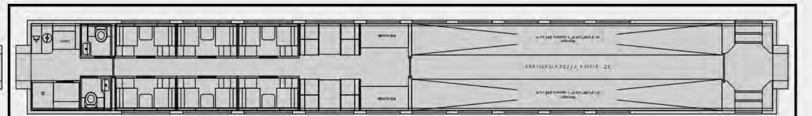
UTILITY CAR - 6 R (Crew) + 8 seats + Minimum of 1,600 cu ft
